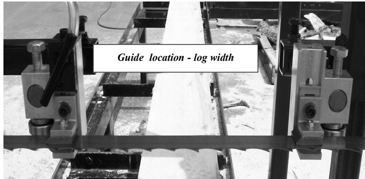
Adjustable blade guide bar and T handle locking bolt.
