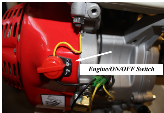
Engine/on/off and start switch
