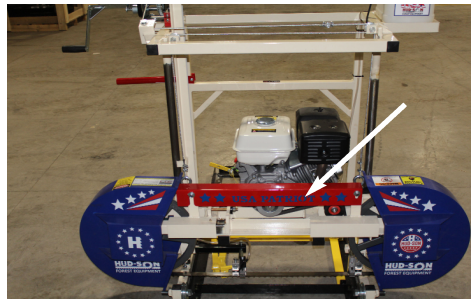
Top blade guard - remove for blade changing
