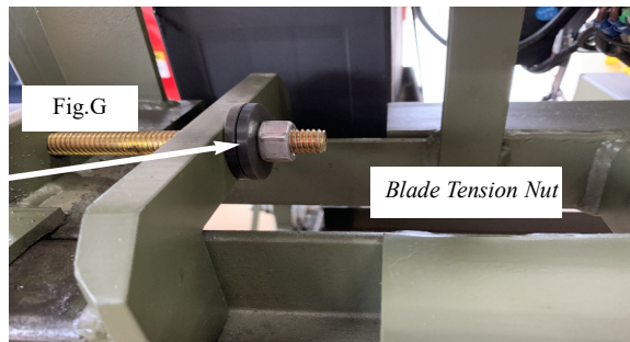
Grease the Blade Tension thrust bearing between the (2) cupped washers .
