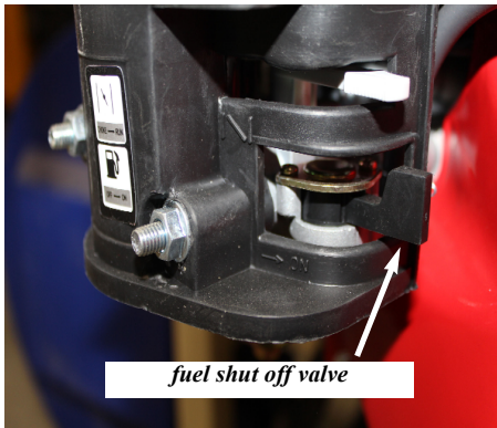
Fuel shut off valve; turn fuel off when not in use
