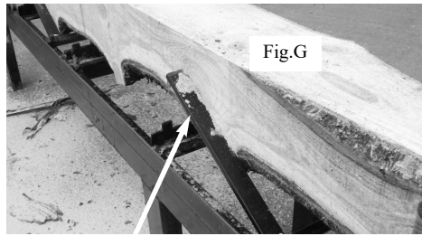
Flat side must be flush and Flat against the squaring pins to assure a square cant.
