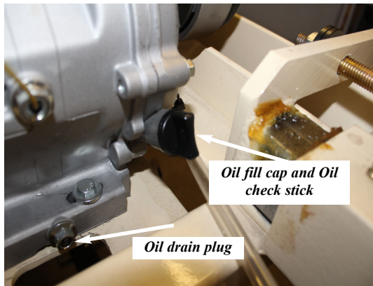
Engine oil check stick and engine oil fill port
